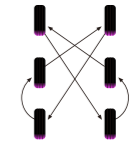
Six wheel three bridge hybrid transposition method
