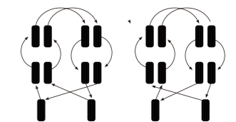
Ten wheel three bridge cyclic transposition method
